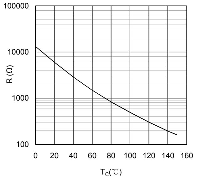
Figure 13. NTC Characteristics
